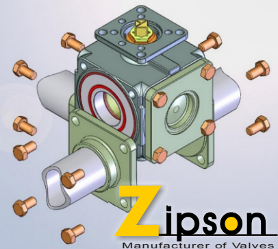
Item 505T, Multi-Way Ball Valve In-Line Repairable Type (3)
